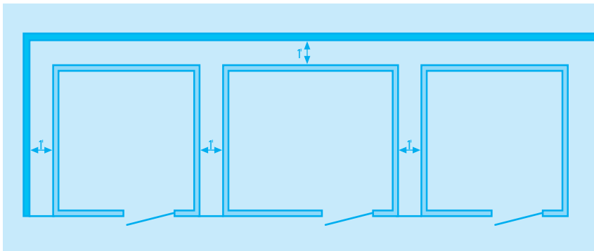
Typical plan view of a sound-isolation room installation. One foot of space recommended between rooms for optimum acoustical performance.
